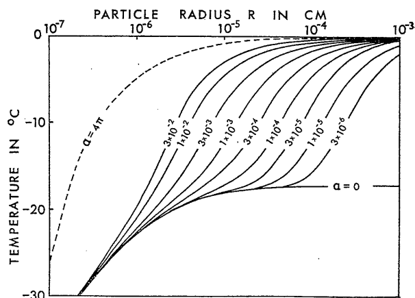
FIG. 2. Freezing nucleation behavior of a particle with surface parameter m=0.5 and having an active site of area \alpha R^2 .
