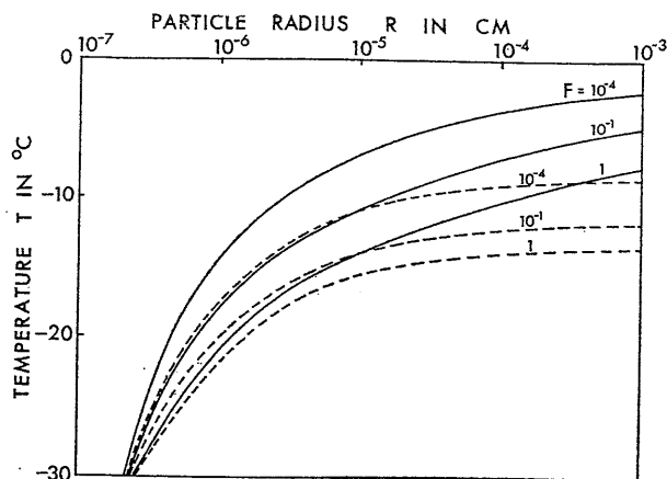
Fig. 4. Curves showing temperature T above which a fraction F of particles of radius R are active as freezing nuclei. The full curves are for \gamma=0.8 , \beta=0.001 and the broken curves for \gamma=1.0 , \beta=0.001 . The value of F is shown as a parameter.
